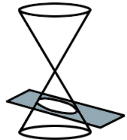
Ellipse
